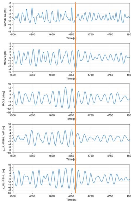
Time traces of incident wave, heave, roll and transverse and vertical motion of the bilge area portside ( H_s = 6.5\text{ m} , T_p = 14.5\text{ s} , wave direction=270 deg, V_s = 0\text{ kn} )
